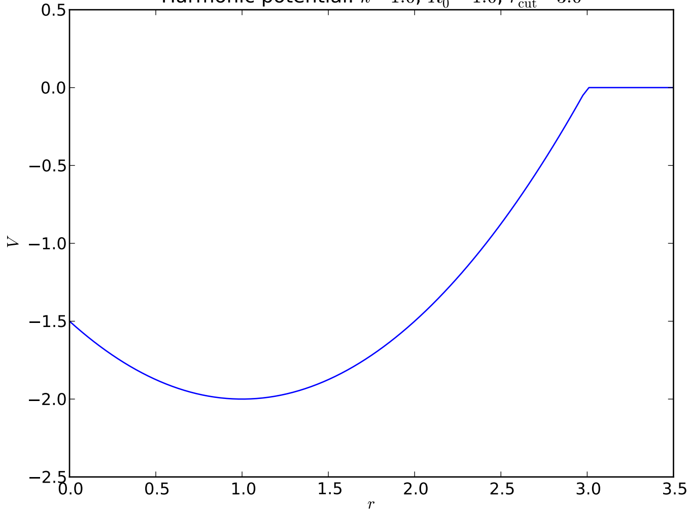
Harmonic potential: k=1.0 , R_0=1.0 , r_{\text{cut}}=3.0
